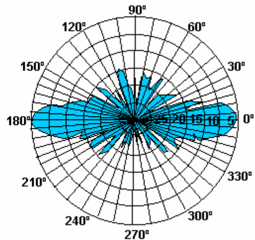
Vertical Beamwidth 20°
