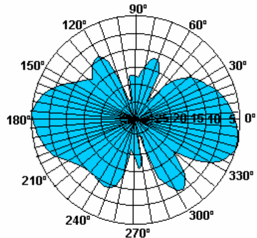
Vertical Beamwidth 28°
